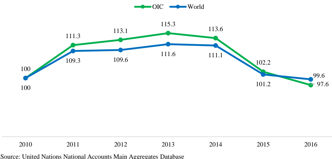
Figure 13.2: GDP Deflator (2010 = 100), 2010-2016
