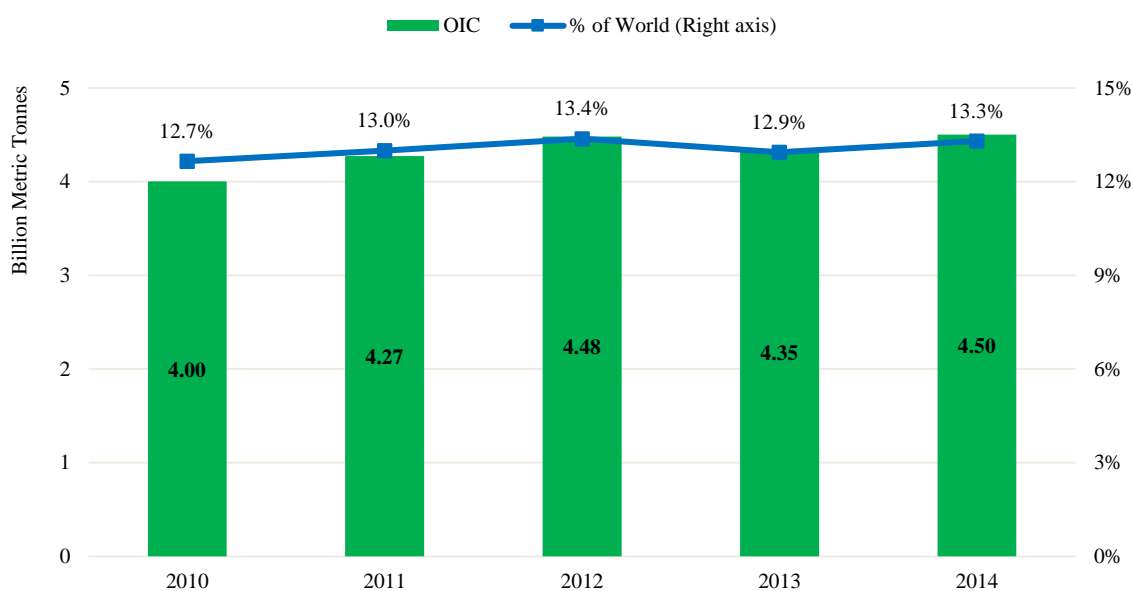
Figure 5.1: CO 2 Emissions, 2010-2014
